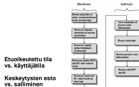
Figure 1.10 Simple Interrupt Processing
