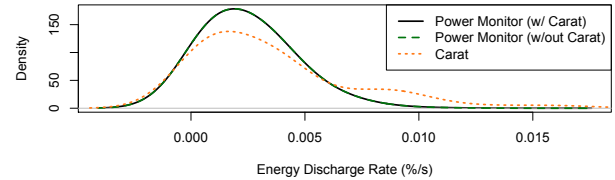
Figure 13. The energy rate distributions from our iOS power metering experiments, smoothed with a Gaussian kernel estimator for visibility. Using the a priori , Carat is able to faithfully estimate the distribution with sparse sampling, overestimating the mean energy drain rate by only 0.00088% from 9 samples.
