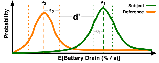
Figure 3. We compare distributions of the expected values of battery drain to identify anomalies ( d' > 0 ) and quantify the error and confidence ranges for expected battery drain under different conditions.
