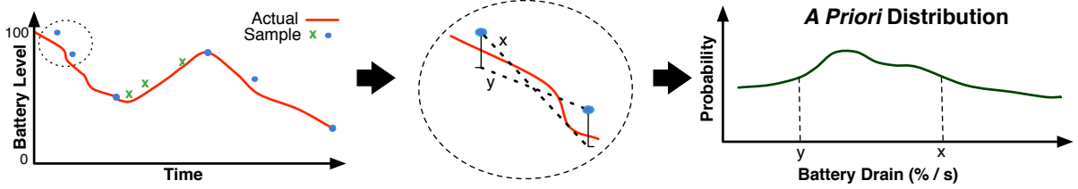
Figure 2. The process of converting battery level samples to rate distributions using the a priori distribution. Samples marked with green Xs are discarded because the device was charging. iOS may report a battery level up to 5% above the actual level. The slope bounds ( x and y ) determine the a priori slice.
