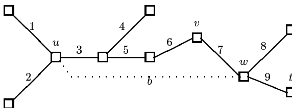
Fig. 1: Example tree.
