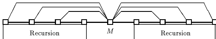
Fig. 2: Construction for diameter 2.
