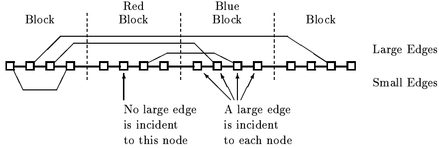
Fig. 5: Lower bound for diameter 3.
