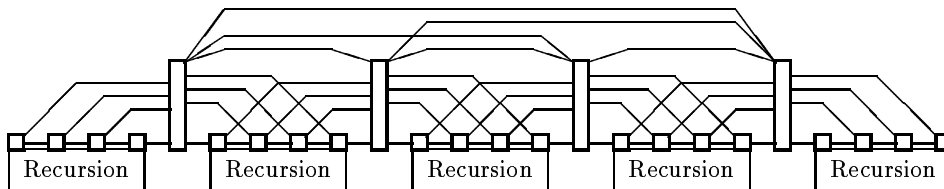
Fig. 4: Construction for diameter 3.
