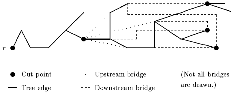
Fig. 8: Upstream and downstream bridges.
