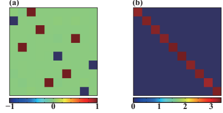
Figure 1: Artificial data, Case 1 (independent sources): (a) Estimated performance matrix \mathbf{P} . \mathbf{P} is re-scaled so that its absolute maximum value is one. (b) Dependency matrix \mathbf{M} .
