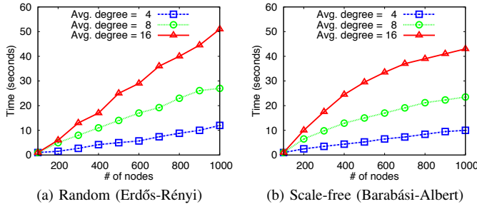
Fig. 4: Time to construct synthetic networks of different type.
