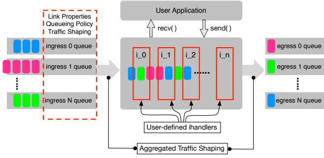
Fig. 3: Logical structure of SRouter
