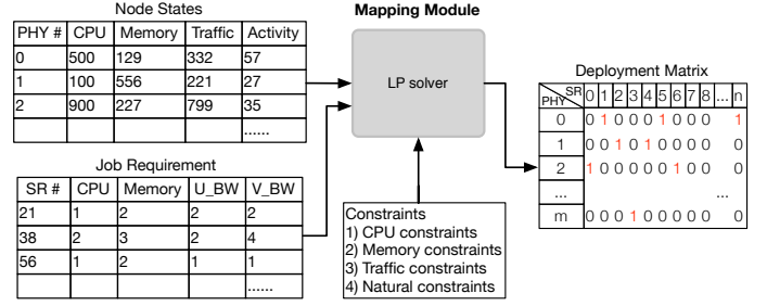
Fig. 2: Inputs and output of Mapping module
