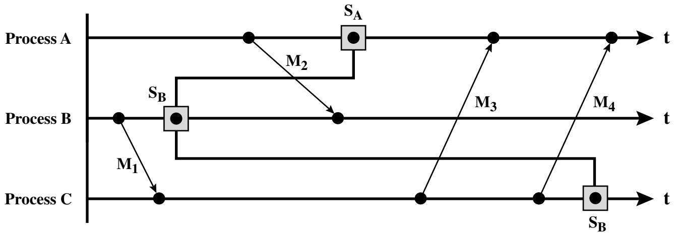
(b) Consistent Global State
