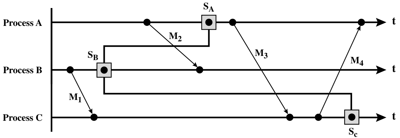
(a) Inconsistent Global State
