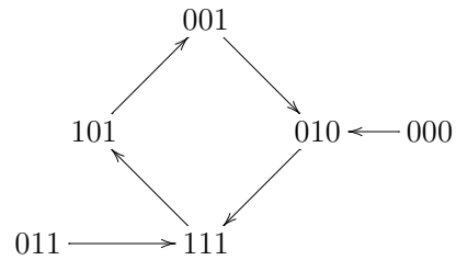
Figure 3: The state transition graph of the Boolean network of Figure 1.
