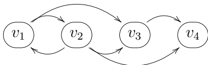
Figure 4: A Boolean network example with four genes v_1, \dots, v_4 and six edges.
