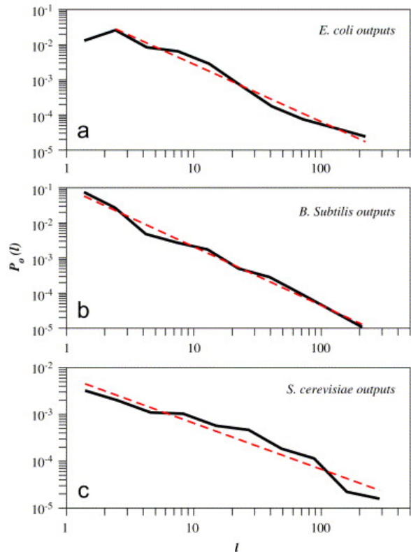
Figure 7: Target distribution for (a) E.coli , (b) B.subtilis , and (c) S.cerevisiae . The solid line corresponds to the experimental data and the dashed lines to distributions that approximate the data well, that are, power law distributions with (a) \gamma \approx 1.636 , (b) \gamma \approx 1.673 , and (c) \gamma \approx 0.984 . All graphs are in log-log scale. Source: [4].
