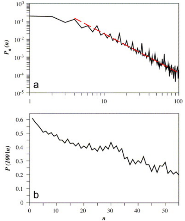
Figure 16: (a) Probability p_a(n) that the original network has n attractors. (b) Conditional probability p(100|n) that all attractors are conserved given that there were n attractors in the original network. For both, (a) and (b) a scale-free topology, 200 genes, k = 2 , and 20,000 network realizations were used. Source: [4].
