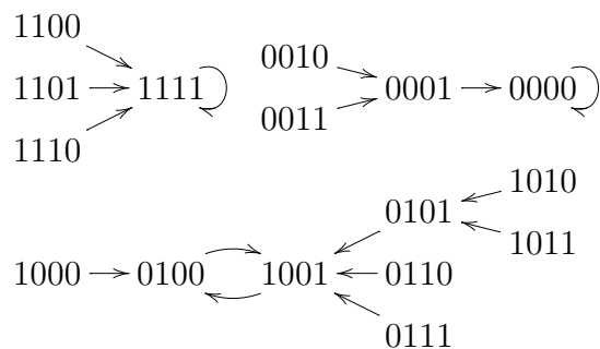
Figure 5: The attractor landscape of the Boolean network in Figure 3 as a state transition graph.
