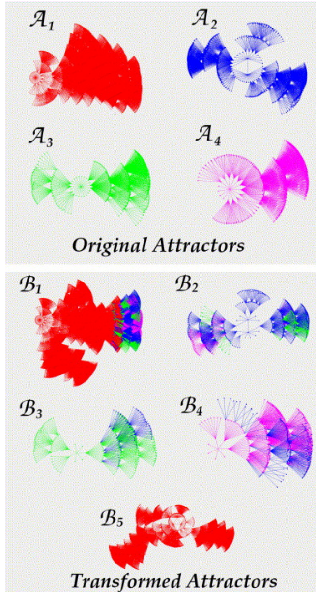
Figure 17: Attractor landscapes of an exemplary network with k = 2 and |V| = 15 before (original attractors) and after (transformed attractors) duplication and divergence of one gene. The original attractors ( \mathcal{A}_1, \dots, \mathcal{A}_4 ) are conserved ( \mathcal{B}_1, \dots, \mathcal{B}_4 ) and a new attractor ( \mathcal{B}_5 ) emerged. The network states kept their color after the gene duplication and divergence, thus, visualizing the “exchange” of network states between the basins of attraction. Source: [4].
