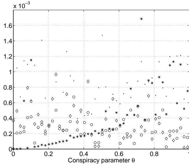
Fig. 1. Mean squared errors of Q at different conspiracy parameters \theta . Lift *, NMF \diamond , PLSA \circ , K-means \cdot .
