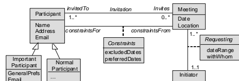
Figure 4.5 – Portion of an entity-relationship diagram for the meeting scheduler
