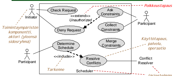
Figure 4.9 – Use case diagram for the meeting scheduler
