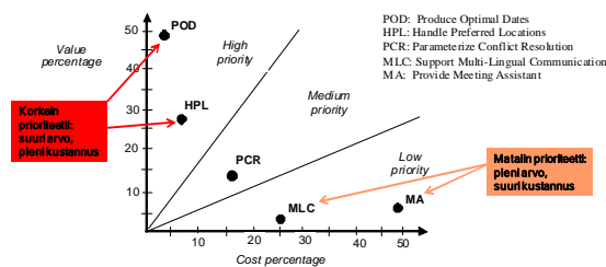
Figure 3.6 – Value-cost requirements prioritization for the meeting scheduler: outcome of the AHP process
