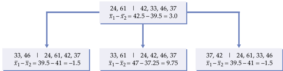
FIGURE 14.20 The idea of permutation resampling. The top box shows the outcomes of a study with four subjects in one group and two in the other. The boxes below show three permutation resamples. The values of the statistic for many such resamples form the permutation distribution.
