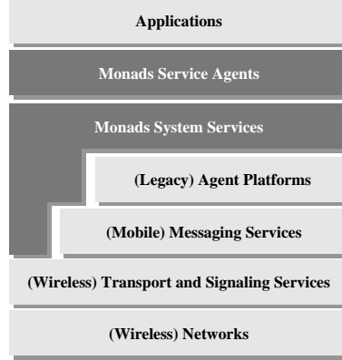
Figure 3: Monads Layered Architecture
