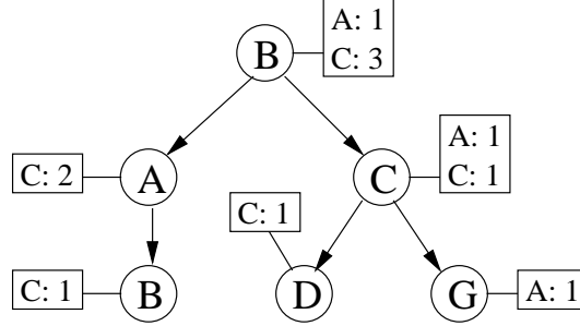
Figure 5: Backward tree for waypoint B.
