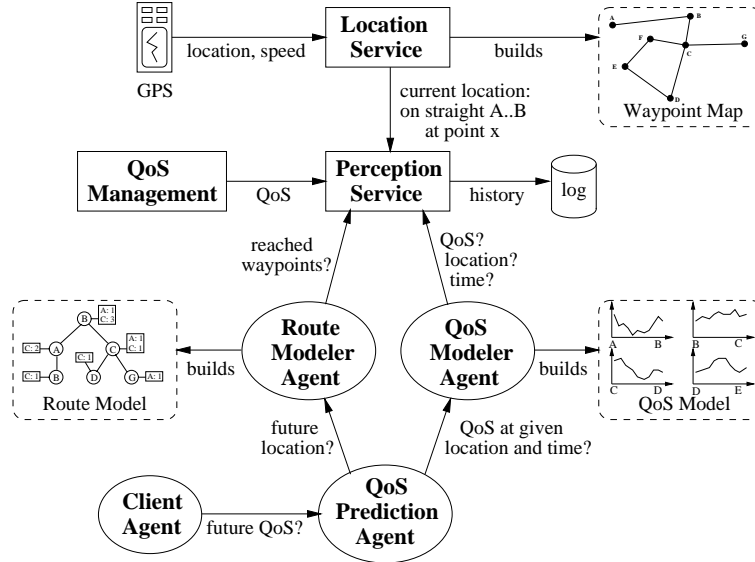
Figure 6: Monads system architecture
