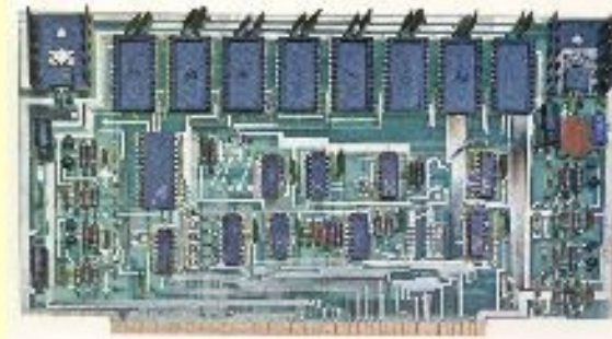
Altair 88-PMC PROM Memory Board
