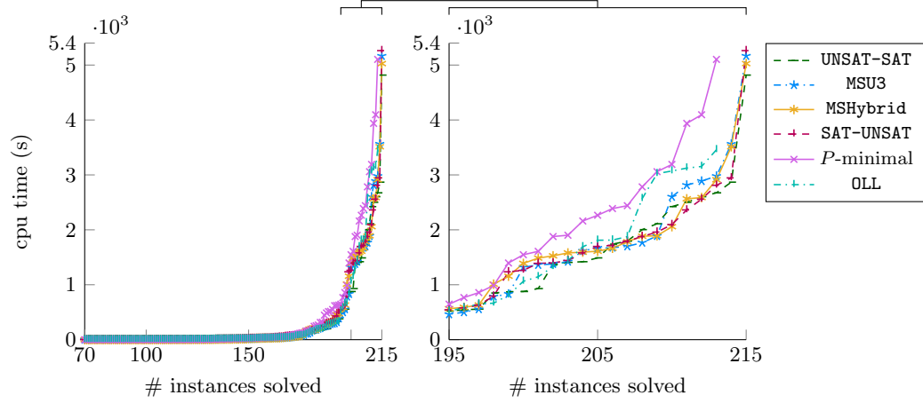
■ Figure 6 Runtime comparison of P -minimal and variants of BiOPTSAT for LIDR on the task of enumerating all solutions on the Pareto front.
