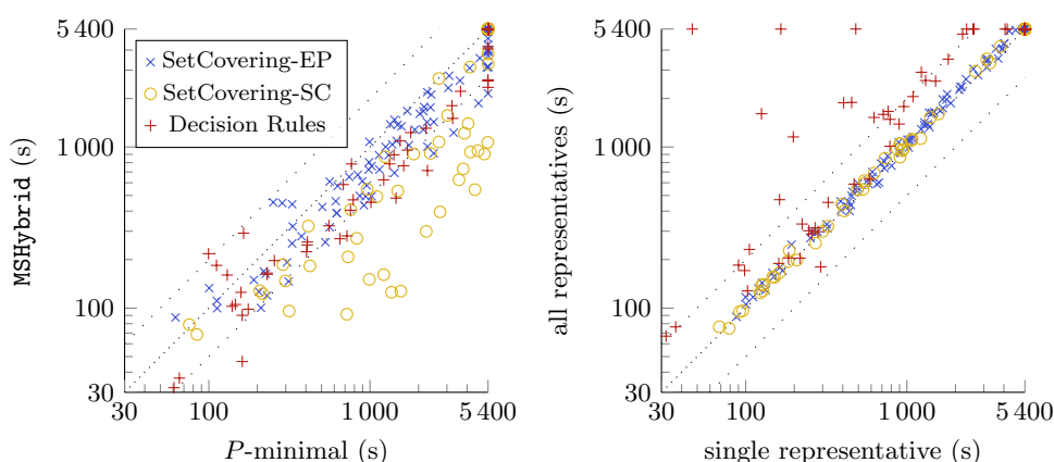
Figure 4 Left: Runtime comparison between P -minimal and BIOPTSAT in the MSHybrid variant. Right: Runtime comparison between enumerating a single representative vs all solutions per Pareto point with MSHybrid.
