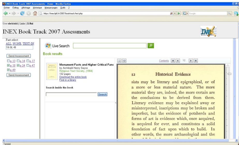
Fig. 5. Screenshot of the Page in Context assessment system. The main frame shows the current book to be assessed, using the Live Search Books service. The frame on the left-hand side of the browser shows the list of pages to be assessed (belonging to the assessment pool). If a page number is clicked on, the corresponding page will display on the main frame. For each book in the pool, the assessor is expected to mark all the relevant pages and submit her assessments. To ease this process, fast selection is provided through “select all”, “select none”, and “text-in” functionalities. While the first two are self-explanatory, the latter offers a simple syntax to select a number of pages with limited effort. For instance, the input “18-36; 49” will cause the automatic selection of all the pages between 18 and 36 (inclusive), as well as page 49.
