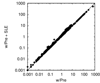
Figure 3: Influence of SLE on preprocessing time
