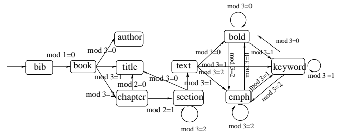
Figure 3: A sample FST for DTD in Fig 2
