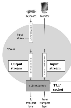
Figure 2.33 TCPclient has three streams
