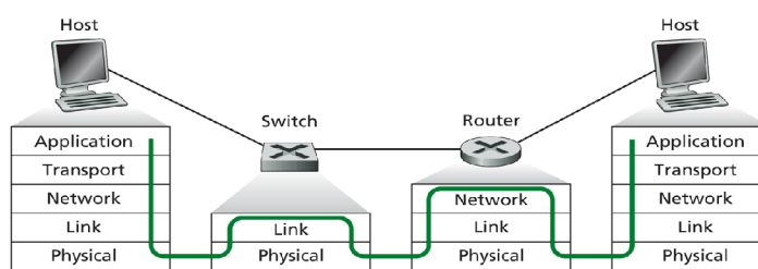
Figure 5.33 ♦ Packet processing in switches, routers, and hosts
