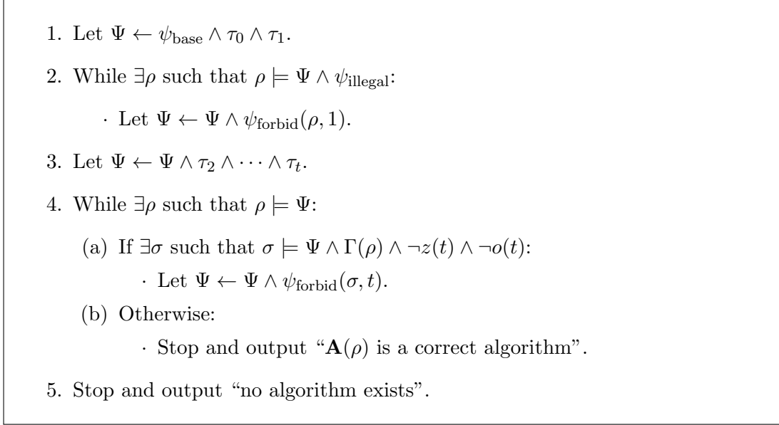
Figure 6: Basic search algorithm. Steps 2, 4, and 4a resort to a SAT solver to find a satisfying assignment of a given formula.
