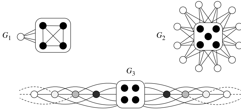
Figure 5: Examples of generalised network topologies. Nodes encompassed within a rectangle form a clique from which the stabilisation propagates throughout the network. Here, G_1 \in \mathcal{G}(4, 3, 1) and G_2 \in \mathcal{G}(5, 3, 1) . The partially illustrated graph G_3 \in \mathcal{G}(4, 3, k) is a cycle where there are additional edges to all neighbours within distance 3.
