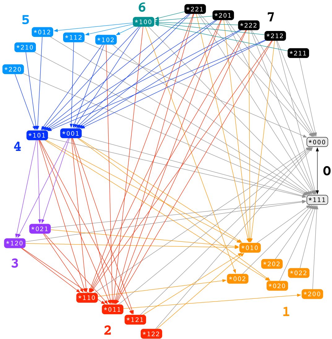
Figure 10: The projection graph G_F(\mathbf{A}) for the algorithm \mathbf{A} given in Table 5, assuming that the faulty nodes are F = \{0\} . The actual configurations have been clustered according to the length of the longest path that avoids the good states \mathbf{0}_F and \mathbf{1}_F . Based on the projection graph, it is straightforward to verify that for any initial state and for any adversarial activities the algorithm will stabilise in t = 7 steps.
