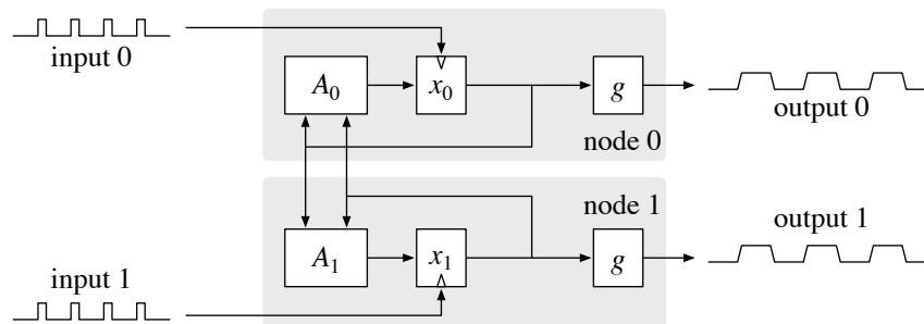
Figure 2: A 2-counter for n = 2 , viewed as an electronic circuit.
