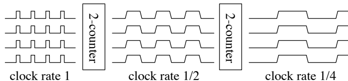
Figure 3: Composition of 2-counters.
