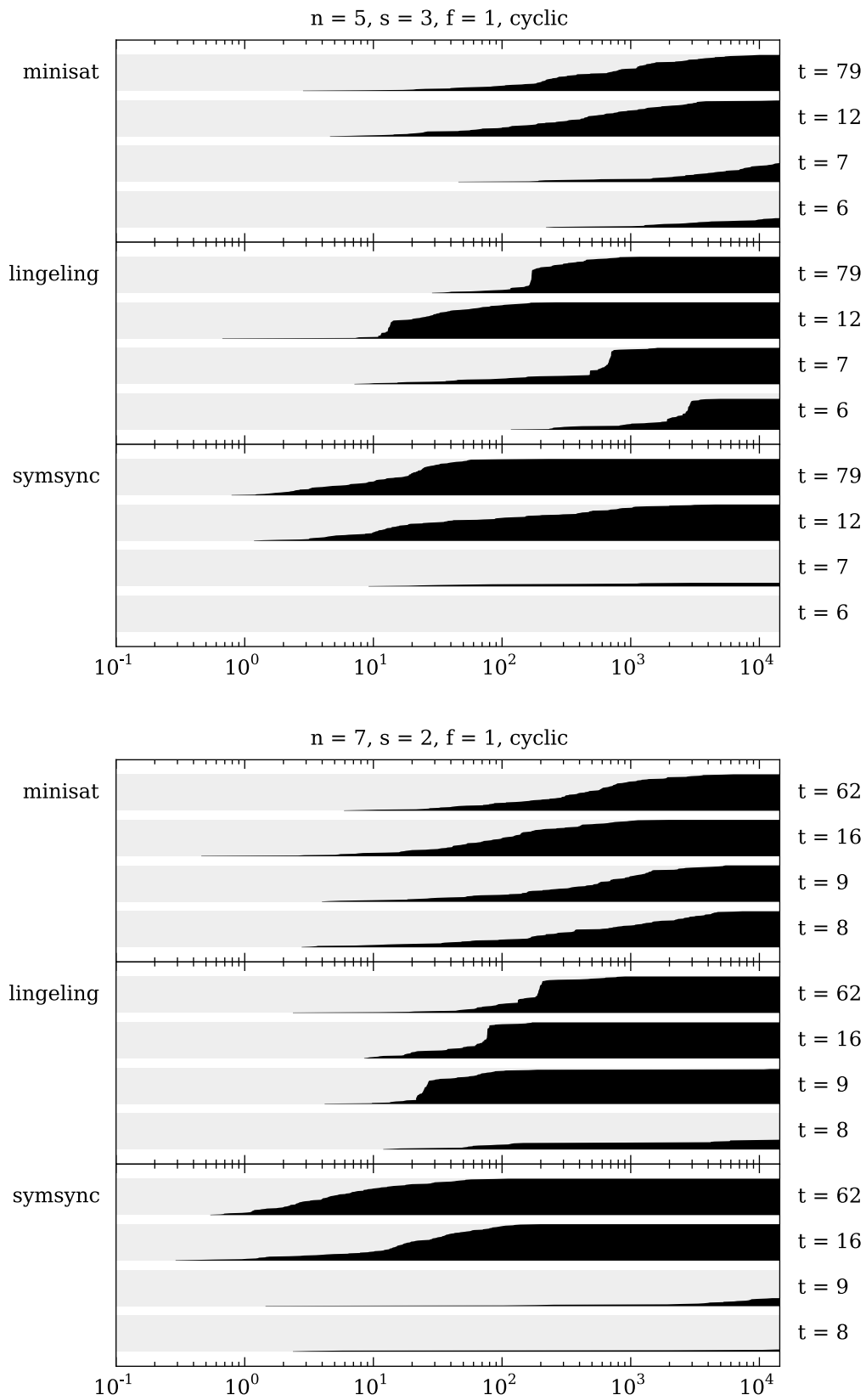
Figure 9: Example of synthesis times. The x axis is the logarithm of time in seconds and the y -axis is the fraction of processes that had solved the problem instance.
