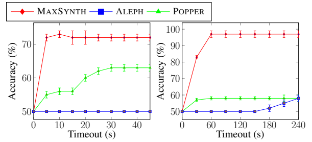
Figure 1: Predictive accuracy with larger timeouts on alzheimer_toxic (left) and zendo2 (20) (right).
