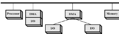
(b) Single-bus, Integrated DMA-I/O
