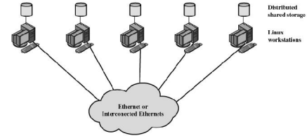
Figure 14.18 Generic Beowulf Configuration
